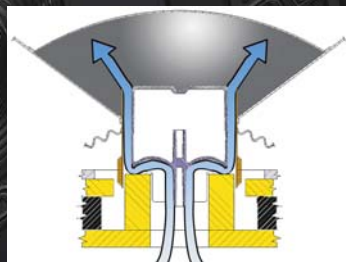
Cool Air Sucked In
